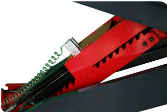
Pneumatic controlled safety lock mechanism
